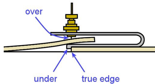
Recess scriber
