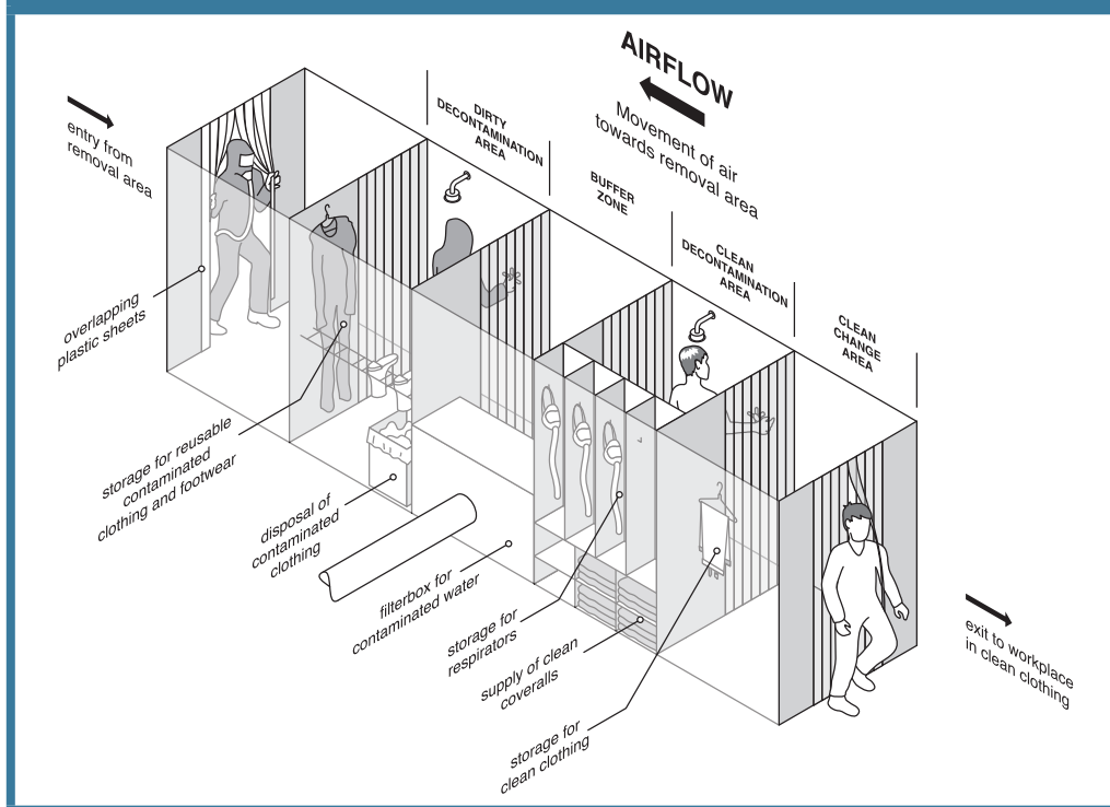
FIGURE 1: Decontamination unit.
